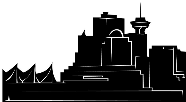
skyline (174)
