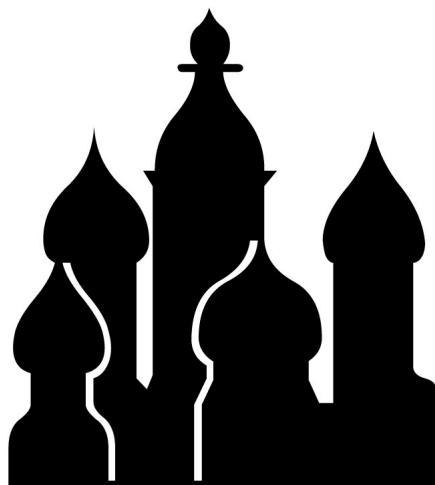
Skyline (8)
